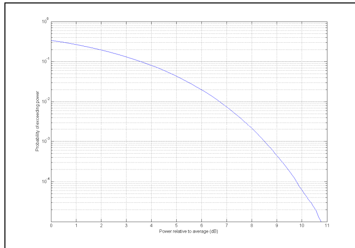
Figure A5: Signal CCDF, showing the probability of exceeding various power levels relative to the average
