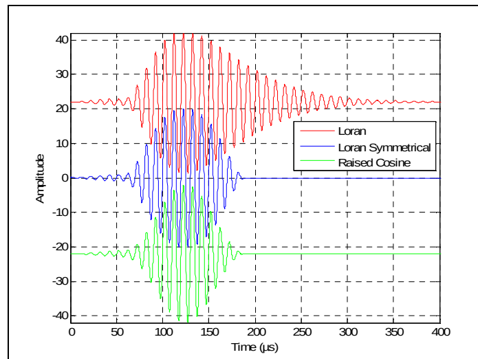
Figure C5: Simulated, received, and composite pulses with 26 dB stronger skywave
