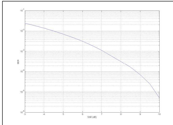
Figure A2: Unencoded bit error rate vs. received SNR for the proposed signal
