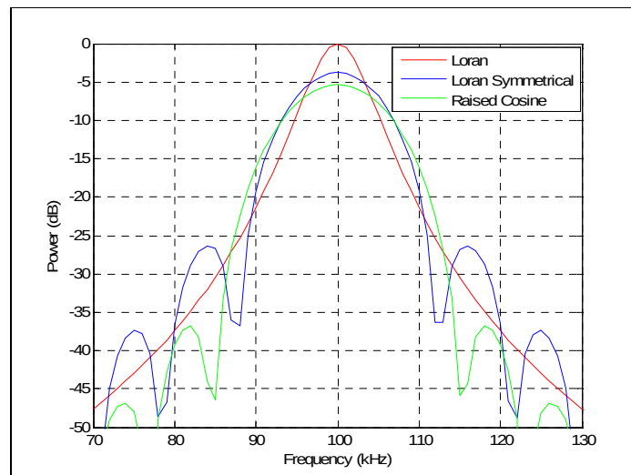
Figure C3: Frequency domain response
