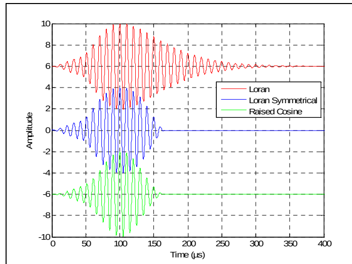
Figure C4: Simulated, received, and composite pulses with 12 dB stronger skywave
