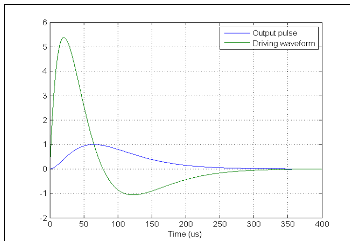
Figure A4: Desired Loran pulse along with the driving waveform required to achieve it into an antenna system with a Q of 60
