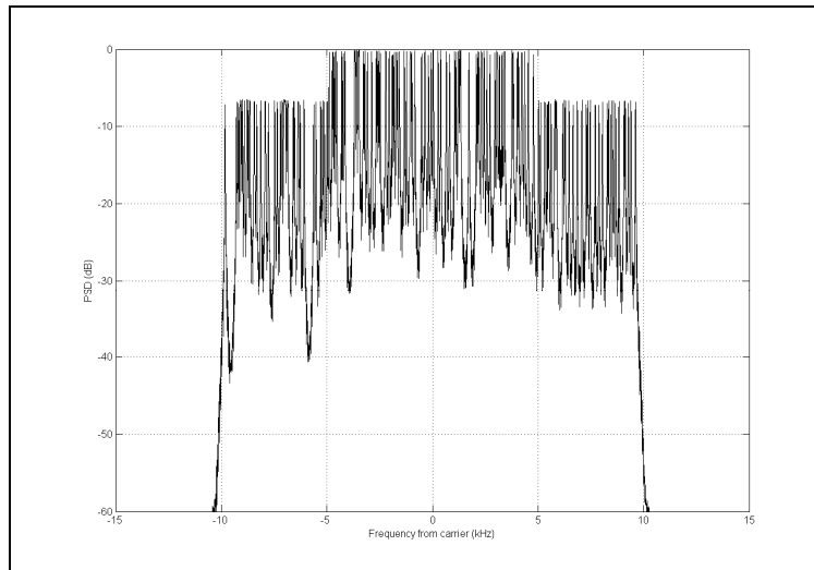
Figure A1: Power spectral density of the proposed signal using a 10 Hz resolution bandwidth
