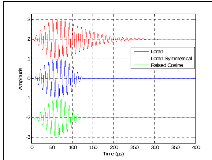
Figure C2: Time domain response
