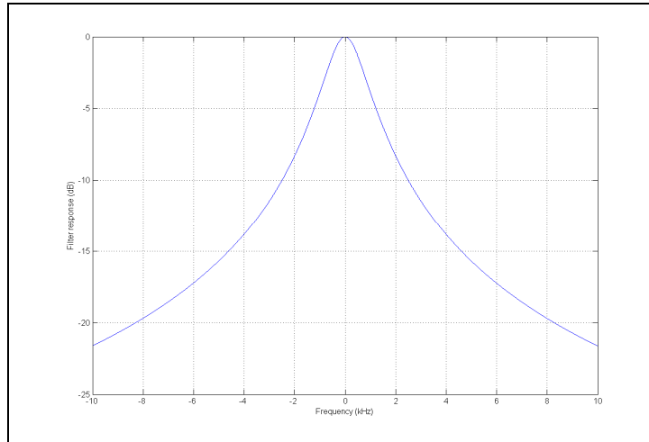
Figure A3: Frequency response of a transmitter filter and antenna with a combined Q of 60
