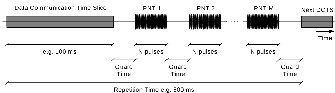
Figure C1: Time sequence of a possible LF PNT&D system
